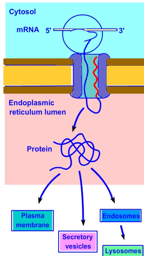
Membrane-bound ribosomes
